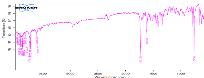
Fig 4: IR spectrum of pure Irbesartan drug
